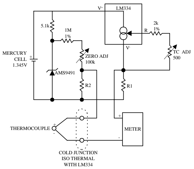
Micropower Thermocouple Cold Junction Compensator
