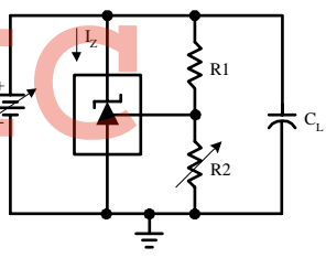
Stability Circuit
