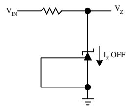
Figure 3. Test Circuit for Off-State Current
