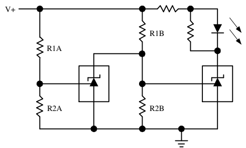
Voltage Monitor
