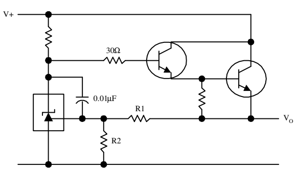
Series Regulator
