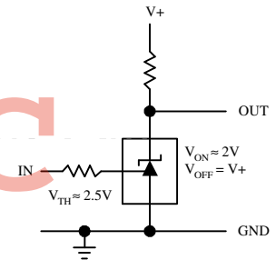
Single Supply Comparator with Temperature Compensated Threshold
