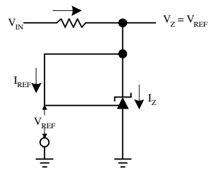
Figure 1. Test Circuit for V_Z = V_{REF}
