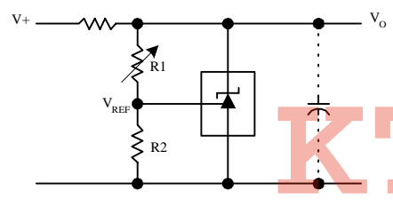
Shunt Regulator
