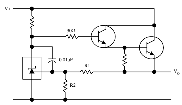
Series Regulator
