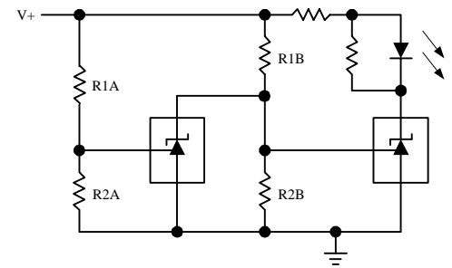
Voltage Monitor
