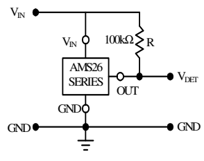
Detector Threshold Test Circuit
