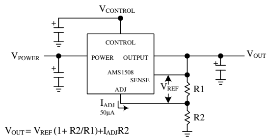
Figure 5. Setting Output Voltage
