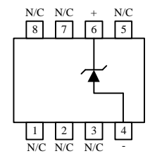
SO-8 SO Package (S)
