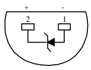
TO-92 Plastic Package (N)
